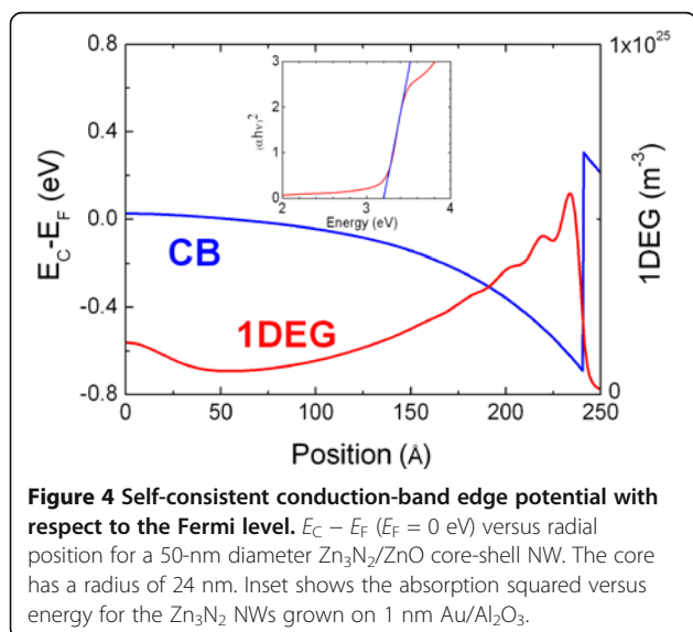
Figure 4 Self-consistent conduction-band edge potential with respect to the Fermi level. E_C - E_F ( E_F = 0 eV) versus radial position for a 50-nm diameter Zn_3N_2/ZnO core-shell NW. The core has a radius of 24 nm. Inset shows the absorption squared versus energy for the Zn_3N_2 NWs grown on 1 nm Au/ Al_2O_3 .
