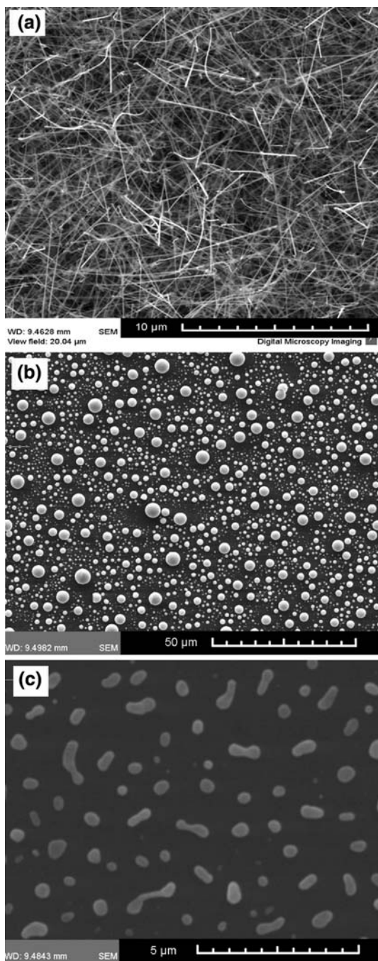
Fig. 1 SEM images of a SnO 2 NWs with an average diameter of 50 nm grown on Au/Si(111) at 800 °C in an inert gas flow of 100 sccm Ar. No droplets exist among the NWs b Sn droplets on Au/Si(111) deposited using the same temperature-time profile in a but in a steady gas flow of 250 sccm of NH 3 as opposed to Ar. A broad distribution in the sizes of the Sn droplets was obtained with diameters \leq 5 \mu\text{m} c similar to b but smaller Sn droplets with diameters \leq 0.5 \mu\text{m} were obtained at 500 °C many of which are also elongated
