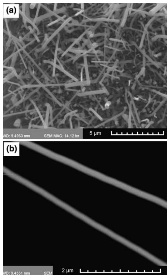
Fig. 2 a \text{Sn}_x\text{N}_y NWs grown on Au/Si(111) at the optimum temperature of 450 °C using a Sn: \text{NH}_4\text{Cl} mixture under a flow of 250 sccm's \text{NH}_3 b high magnification SEM image of \text{Sn}_x\text{N}_y NWs
